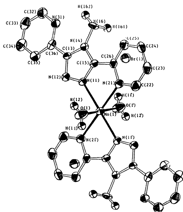
Fig. 1. Projection of [\text{Mn}(\text{C}_{12}\text{H}_{10}\text{N}_6)_2(\text{H}_2\text{O})_2]\text{Br}_2 with the atomic labelling system. Hydrogen atoms that are bonded to carbon atoms are omitted for clarity. Primed atoms are generated by 1 - x, -y, -z .
