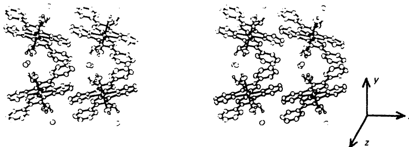
Fig. 2. Stereoview of the packing of [\text{Mn}(\text{C}_{12}\text{H}_{10}\text{N}_6)_2(\text{H}_2\text{O})_2]\text{Br}_2 .
